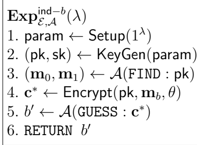
Figure 1: Game for the IND-CPA security of an asymmetric encryption scheme.
